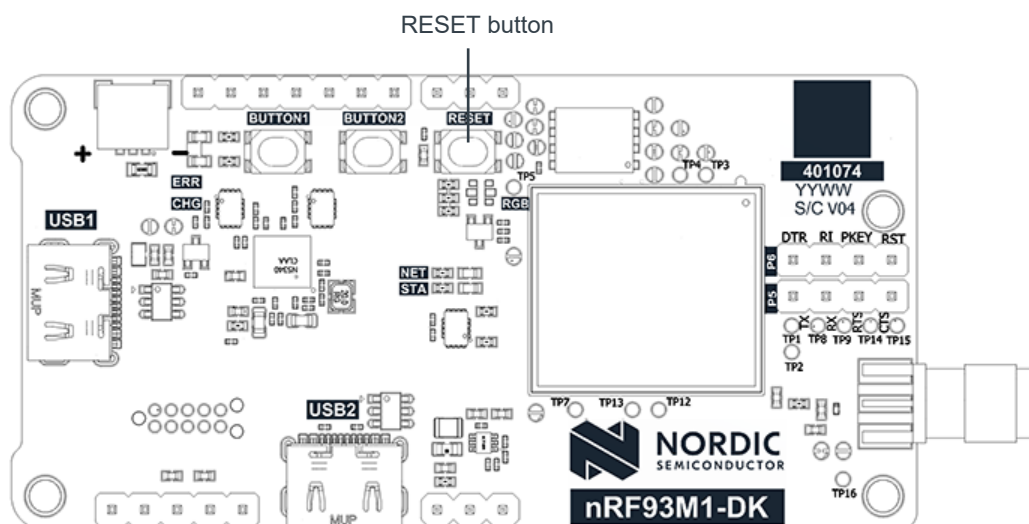
Figure 22: Reset button
