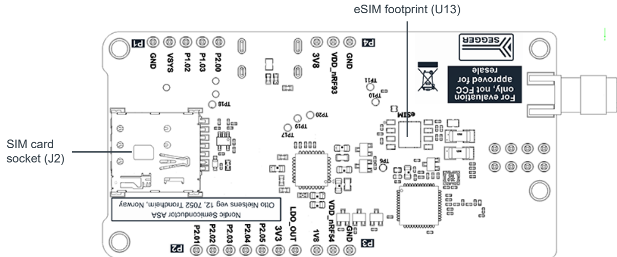
Figure 15: SIM card connector and eSIM
