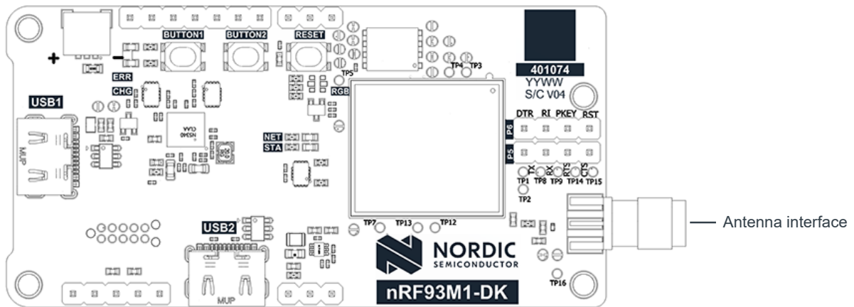
Figure 8: Antenna interface
