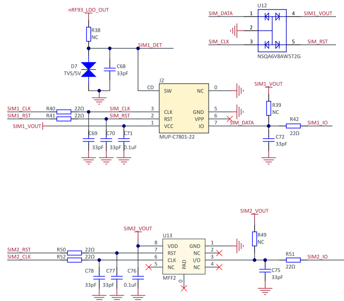
Figure 16: SIM card connector and eSIM
