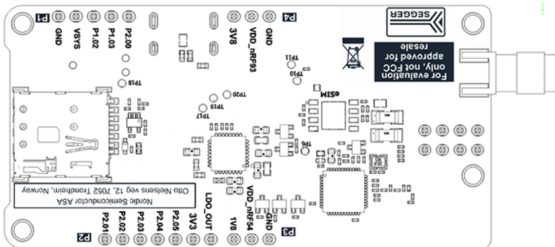
Figure 3: nRF93M1 DK back view
