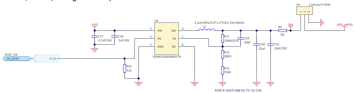
Figure 14: Enable DC/DC regulator
