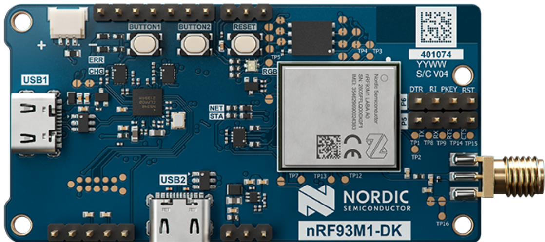
Figure 1: nRF93M1 DK kit content
