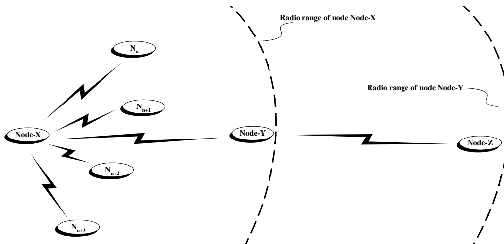
Figure 7 - Network example; System response delay due to retransmission
