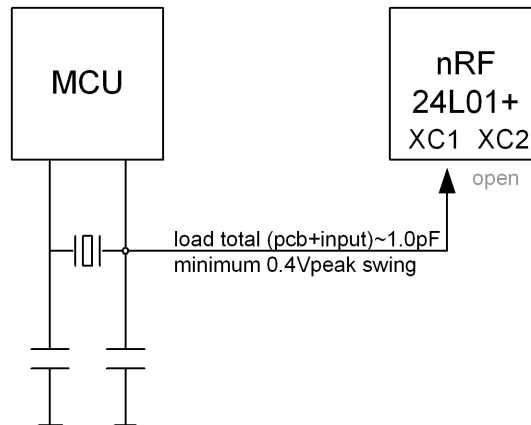
Figure 1. MCU feed nRF24L01+
